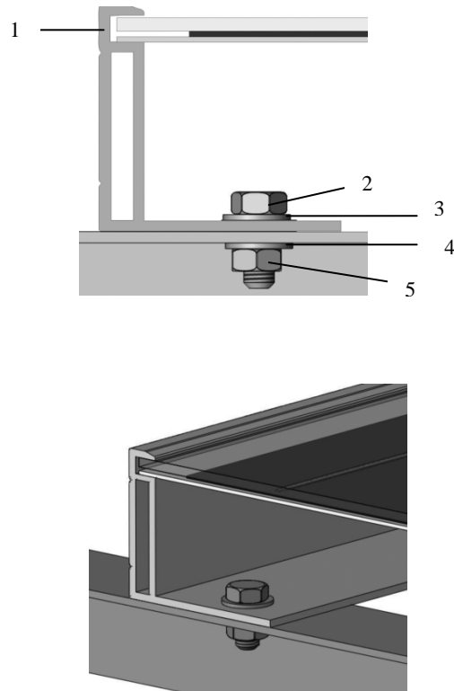
Figure1. SPV module installed with Bolt fitting method
