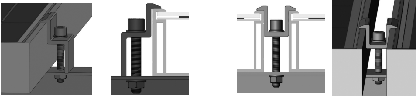
Figure2. SPV module installed with clamp fitting method
